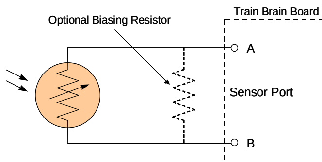
Typical PhotoSensor Schematic
