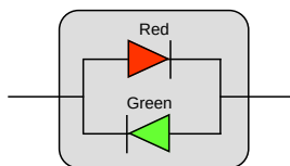
“Bipolar” LED
