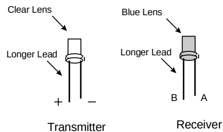
Infrared Components
