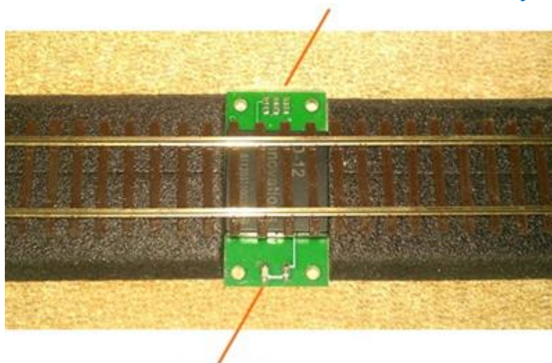
Tag detect LED
