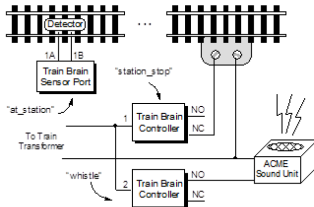
Wiring Diagram for Lesson #3
