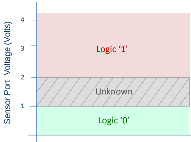
Sensor Port Logic Voltage Regions
