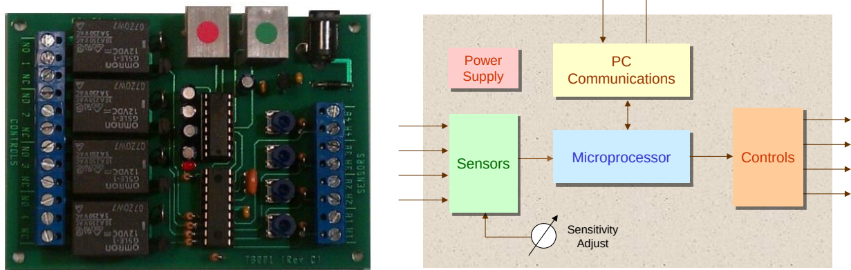
"Train Brain" Module and Block Diagram
