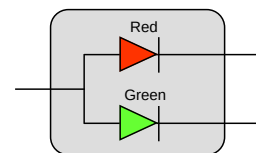
“Bicolor LED” (Common Anode)
